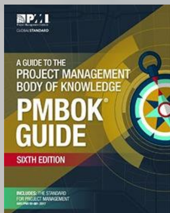
PMBOK 6 th
